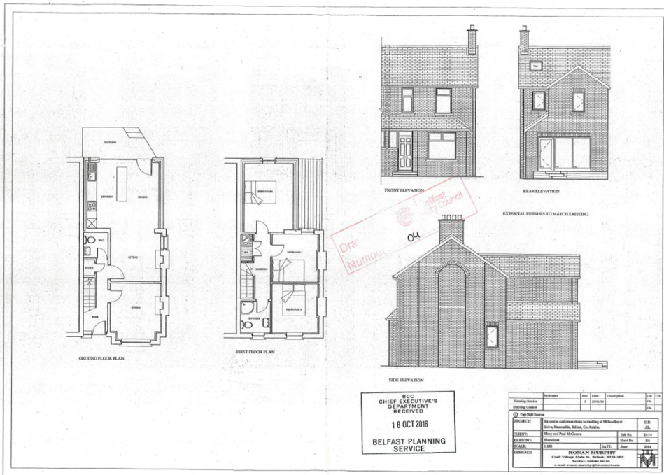
Proposed Elevations / Floor Plans
